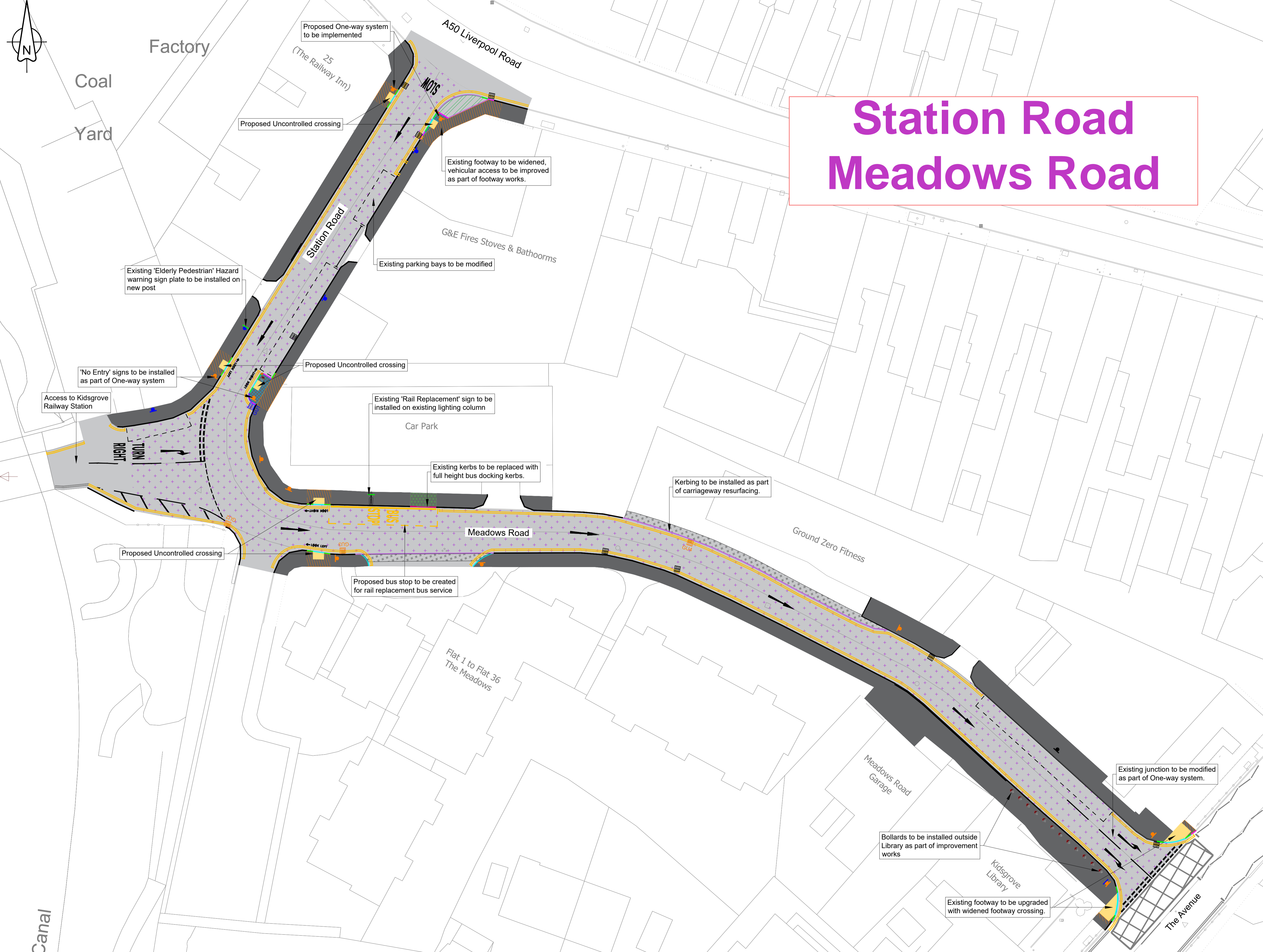
General Arrangement - Station Road/Meadows Road Scale 1:250
